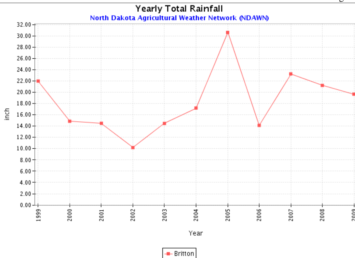
Figure 5. Annual Total Precipitation at Britton, South Dakota from 1999-2009. North Dakota Agricultural Weather Network (NDAWN).
